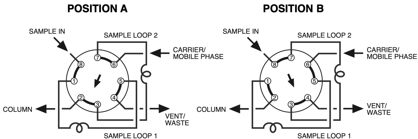
FIGURE 1: Valve viewed from end opposite handle or actuator
