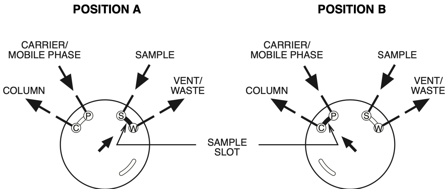
FIGURE 1: Valve viewed from end opposite handle or actuator
