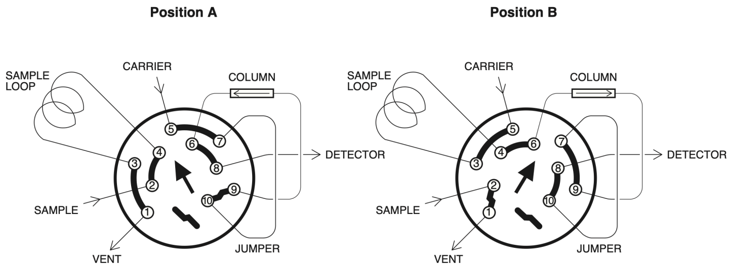
Valve viewed from handle end
