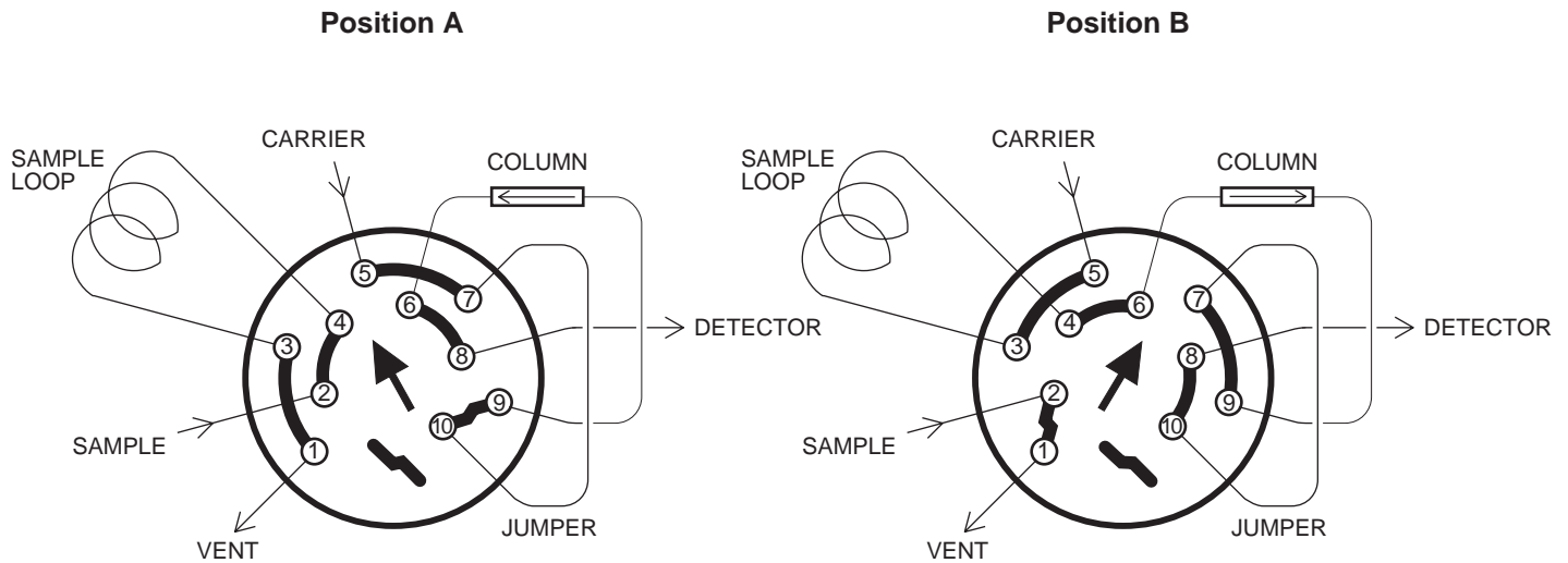
Valve viewed from handle end
