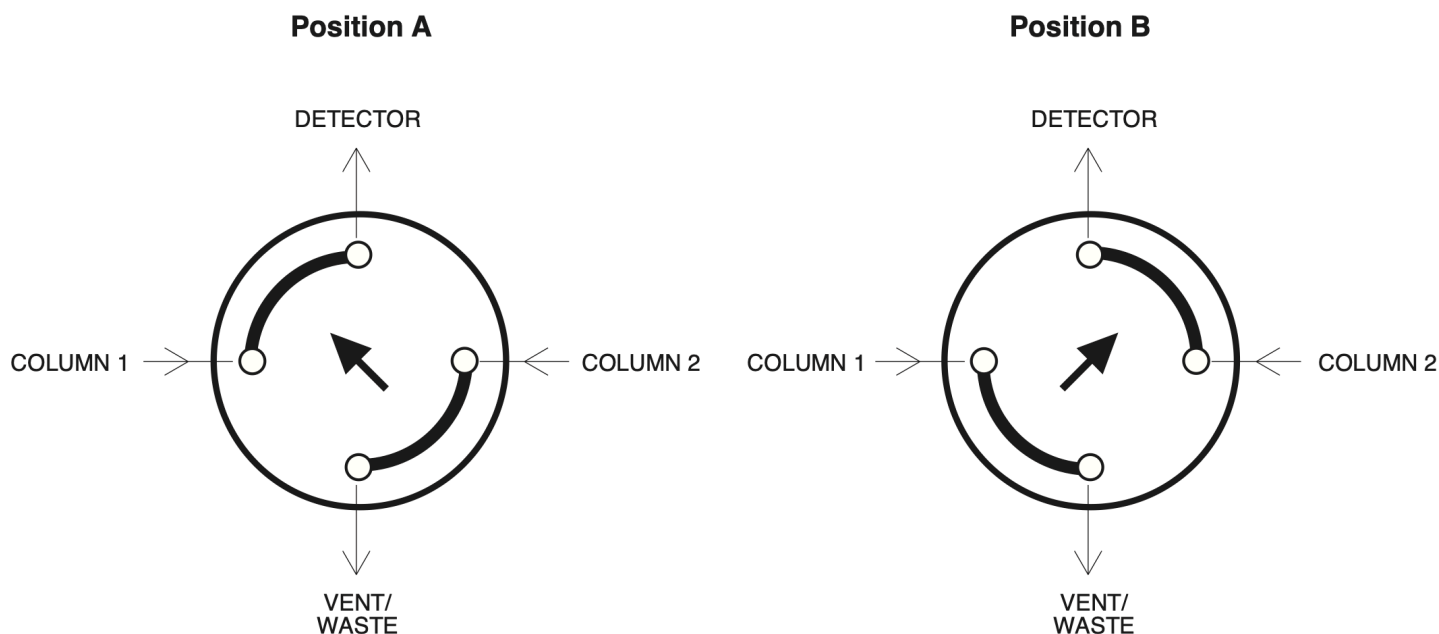
FIGURE 1: Valve viewed from handle end
