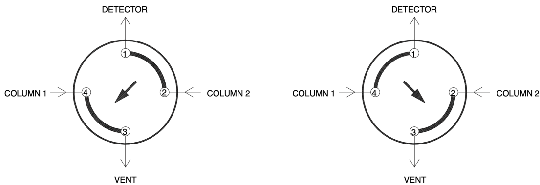
FIGURE 1: Valve viewed from the preload end
