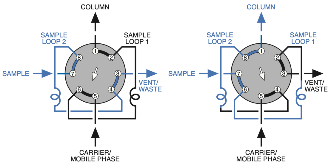
FIGURE 1: Valve viewed from the preload end
