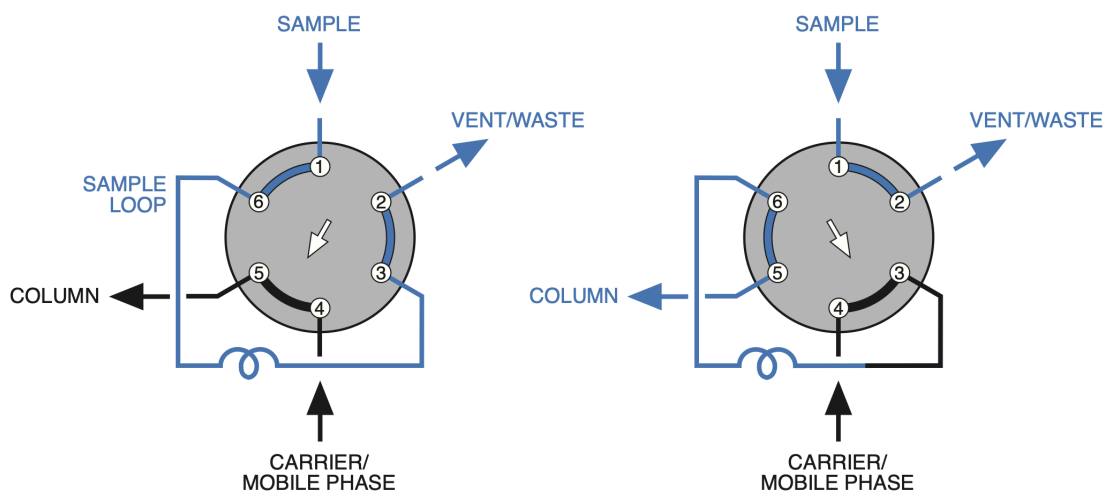
FIGURE 1: Valve viewed from the preload end
